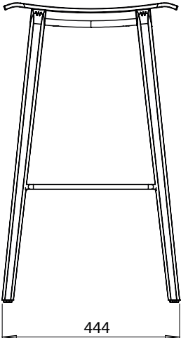
FourWood® Stool 105
