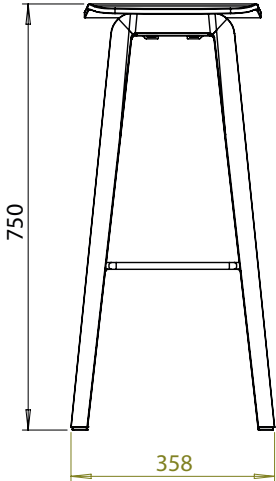
FourWood® Stool 105
