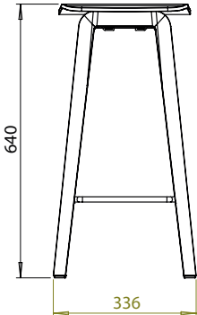
FourWood® Stool 90
