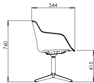
FourMe Lounge, Seat Pad
